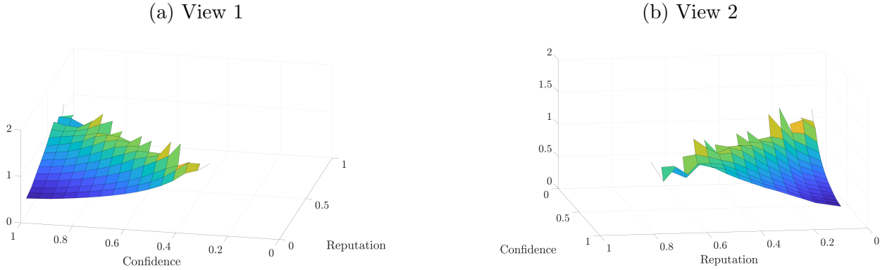
Figure 3: Span
