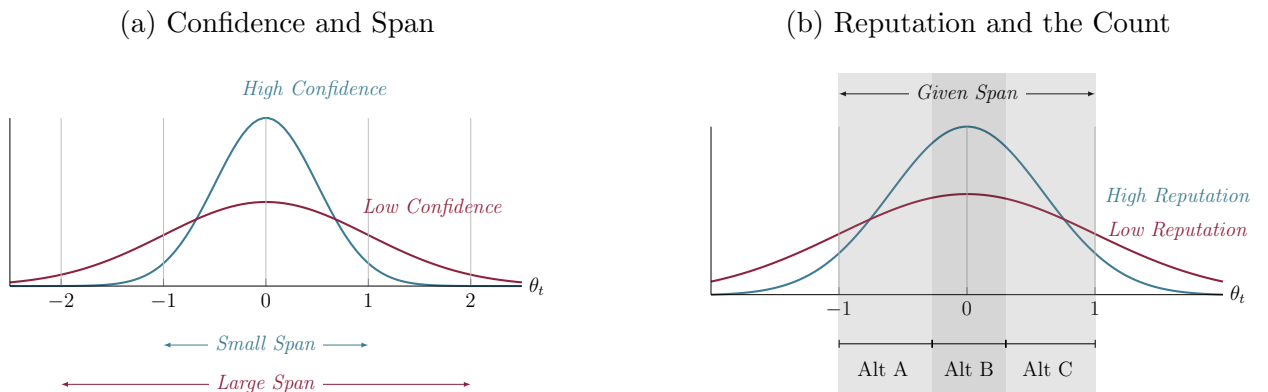
Figure 5: Intuition
