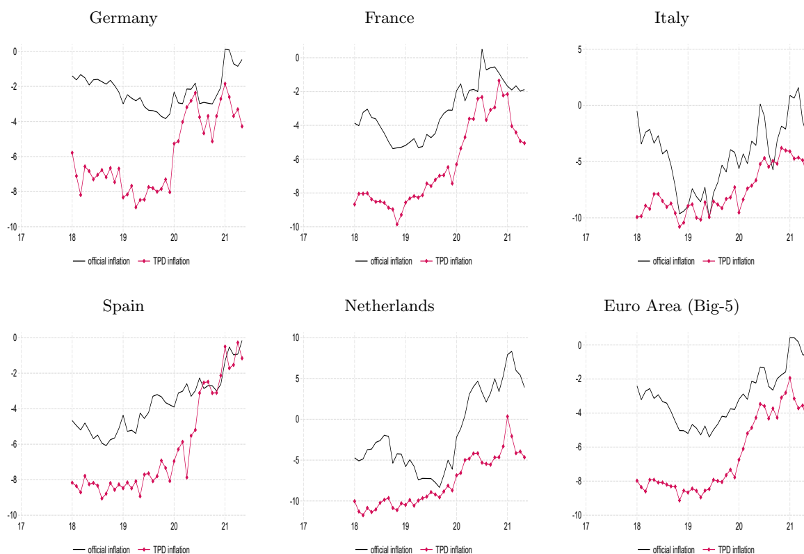
Figure 5: Comparison of official and scanner data-based inflation rates
