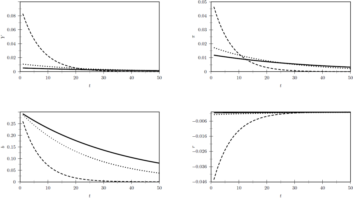
Figure 1: Responses at positive interest rates to a 30% increase in debt outstanding at different durations of government debt.
